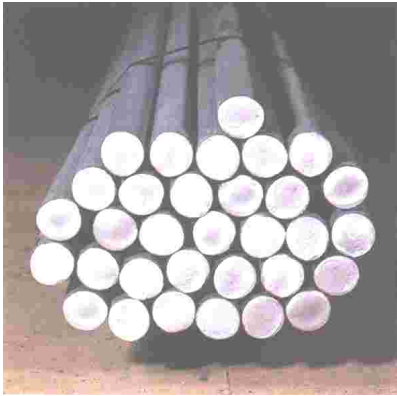
Grinding rods : Ø14mm to Ø100mm 37 HRC
