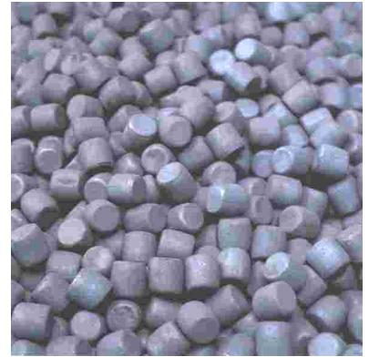
Cylpebs : 8x8mm to 40x40mm 46 – 58 HRC
