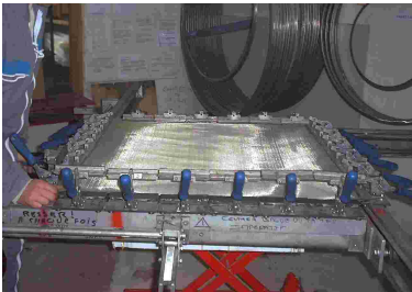
Screen meshing
